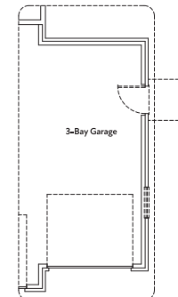
(Optional) 3-Bay Garage
