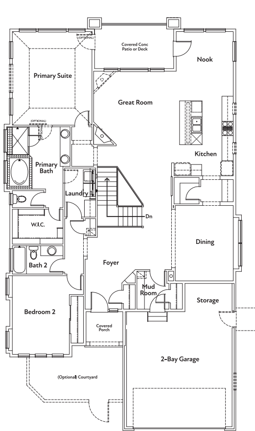
MAIN LEVEL FLOORPLAN
