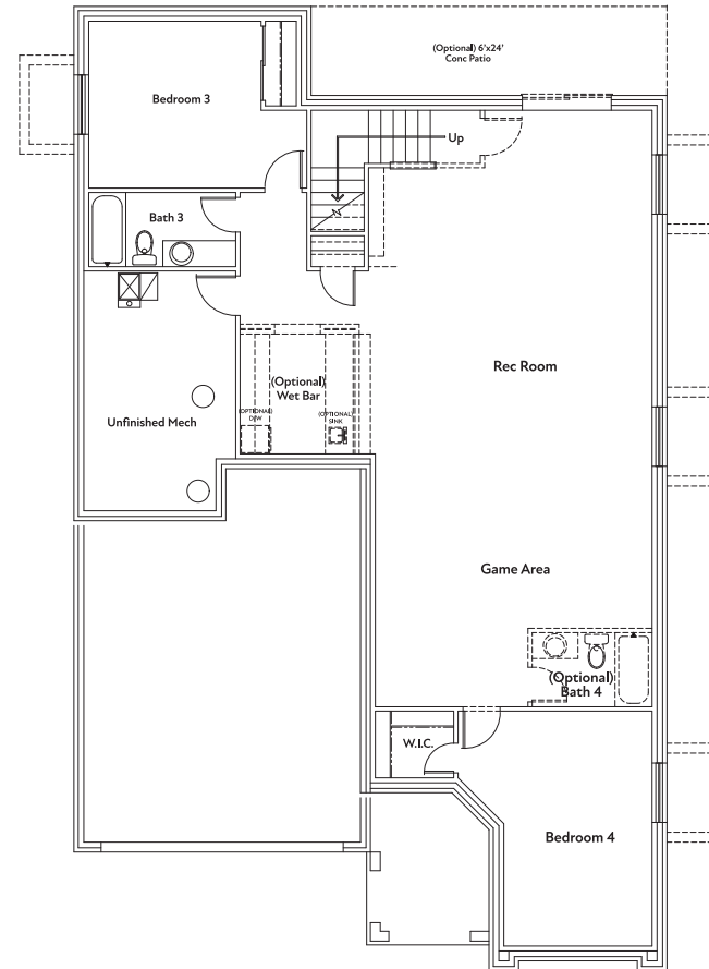
BASEMENT FLOORPLAN
