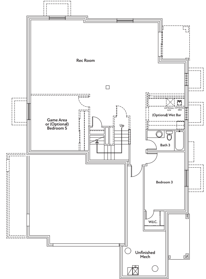
BASEMENT FLOORPLAN
