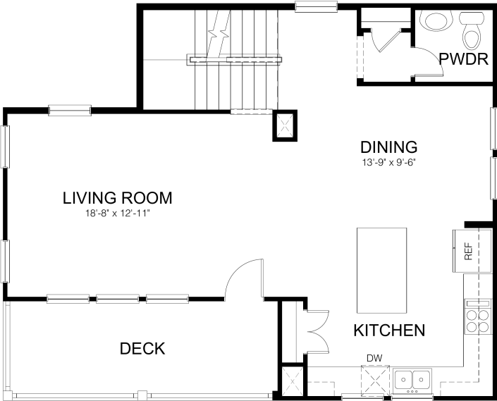
SECOND FLOOR PLAN ELEVATION A
