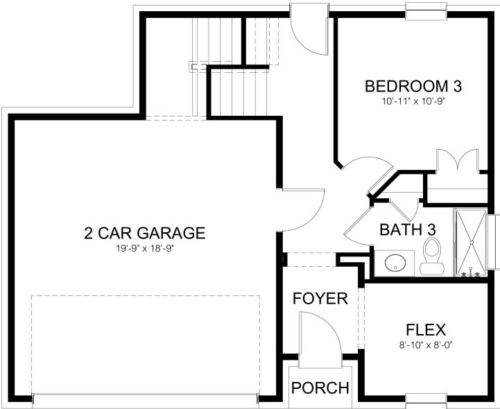
MAIN FLOOR PLAN ELEVATION A
