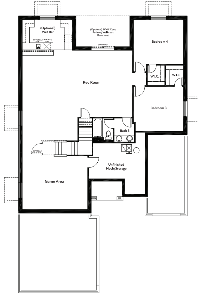
BASEMENT FLOORPLAN
