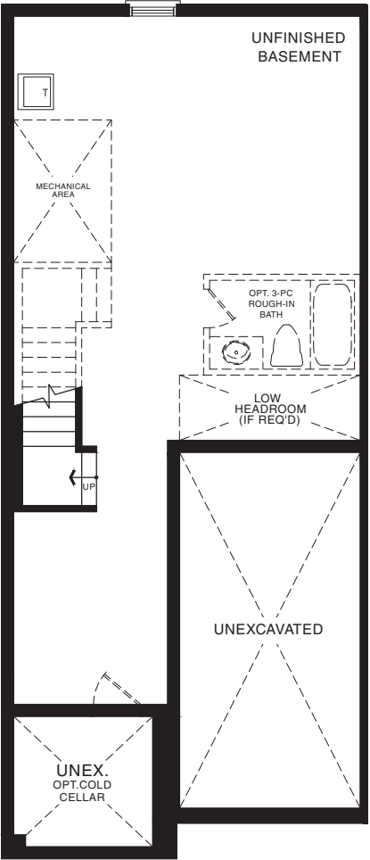
BASEMENT PLAN ELEVATION A1
