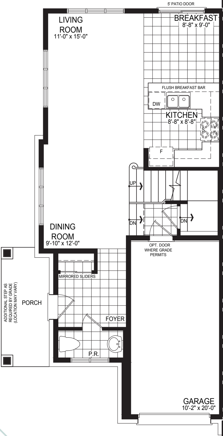
MAIN FLOOR PLAN ELEVATION A1
