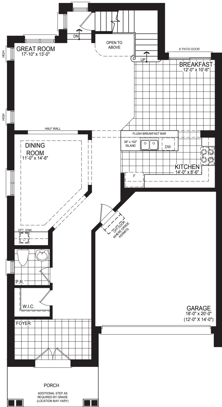
MAIN FLOOR PLAN ELEVATION C
