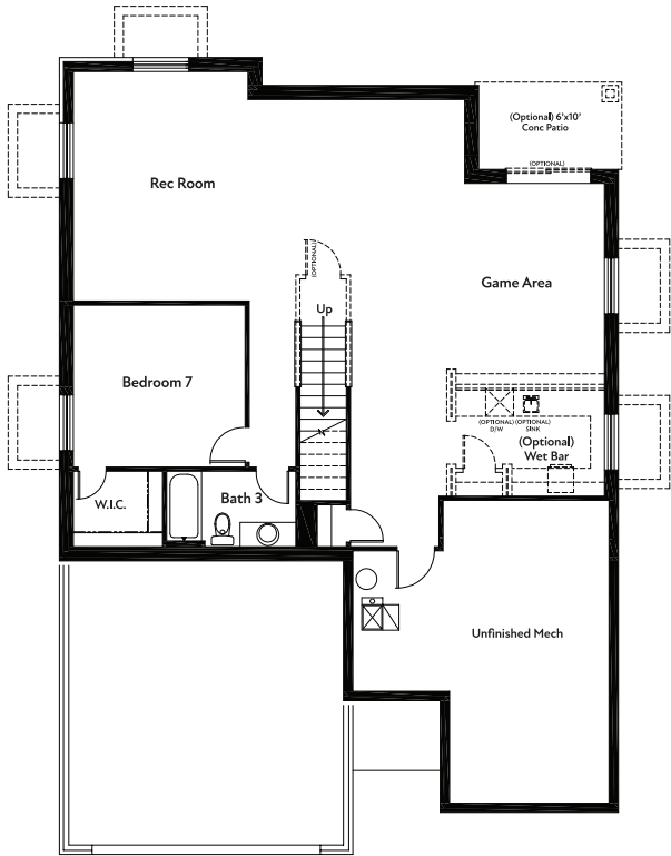
(OPTIONAL) BASEMENT FLOORPLAN
