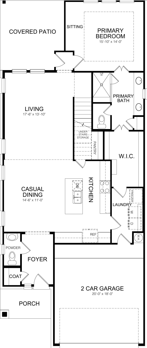
MAIN FLOOR PLAN ELEVATION A
