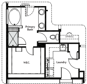
(Optional) 5-Piece Primary Bath
