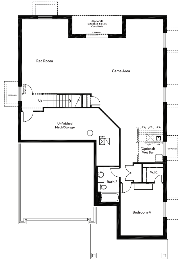
(OPTIONAL) BASEMENT FLOORPLAN
