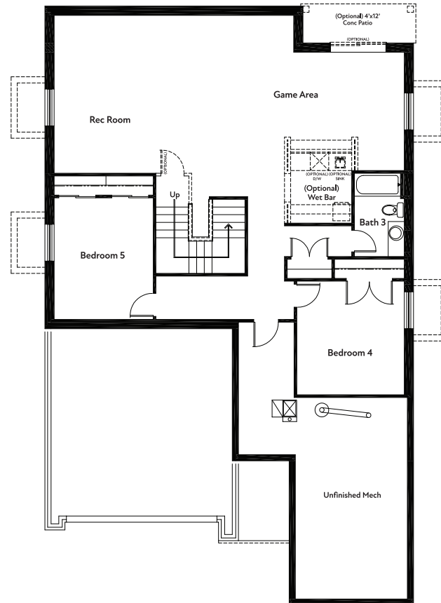
(OPTIONAL) BASEMENT FLOORPLAN
