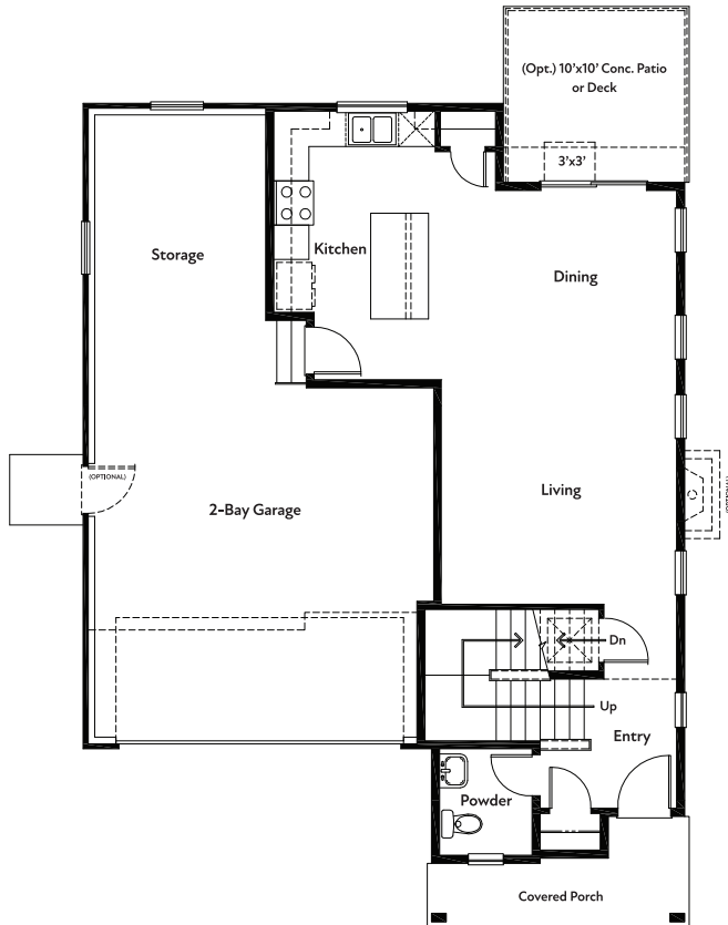
MAIN LEVEL FLOORPLAN
