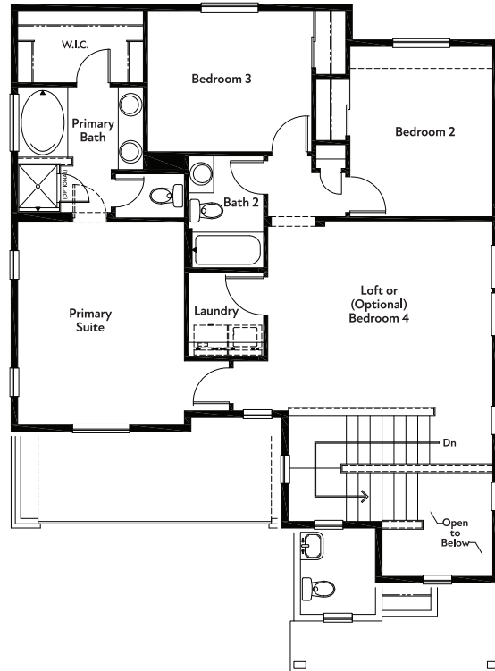
UPPER LEVEL FLOORPLAN
