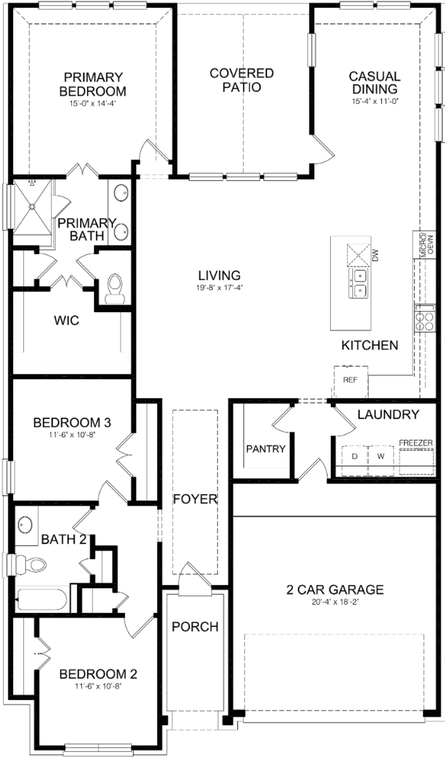
MAIN FLOOR PLAN ELEVATION G
