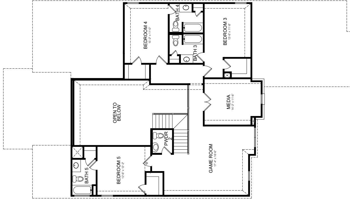
SECOND FLOOR PLAN ELEVATION A
