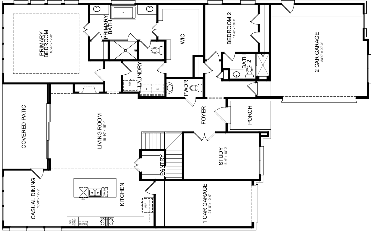
MAIN FLOOR PLAN ELEVATION A
