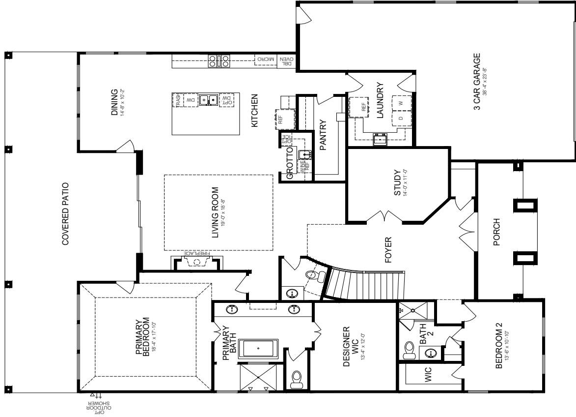
MAIN FLOOR PLAN ELEVATION A
