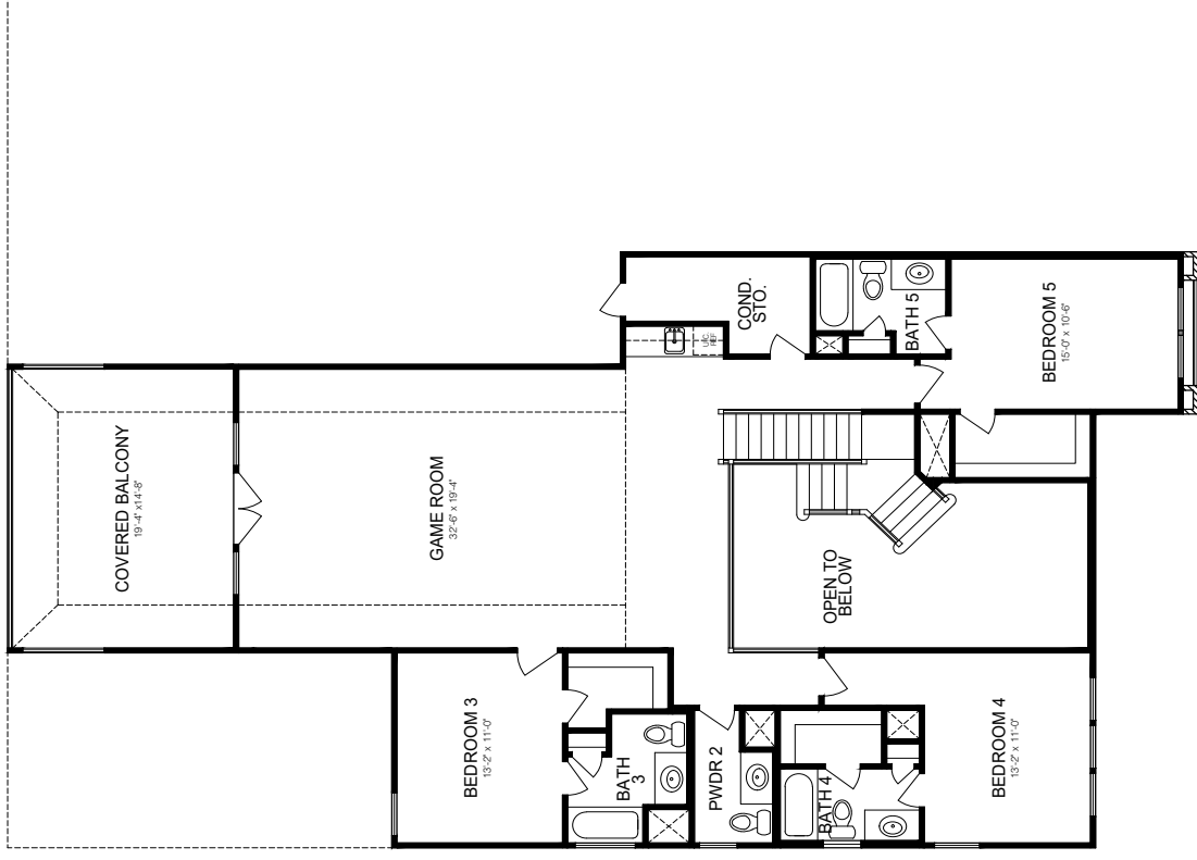
SECOND FLOOR PLAN ELEVATION A
