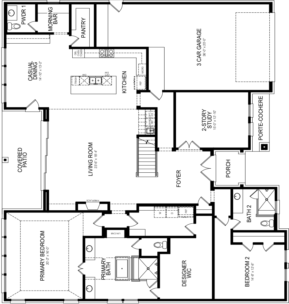
MAIN FLOOR PLAN ELEVATION A
