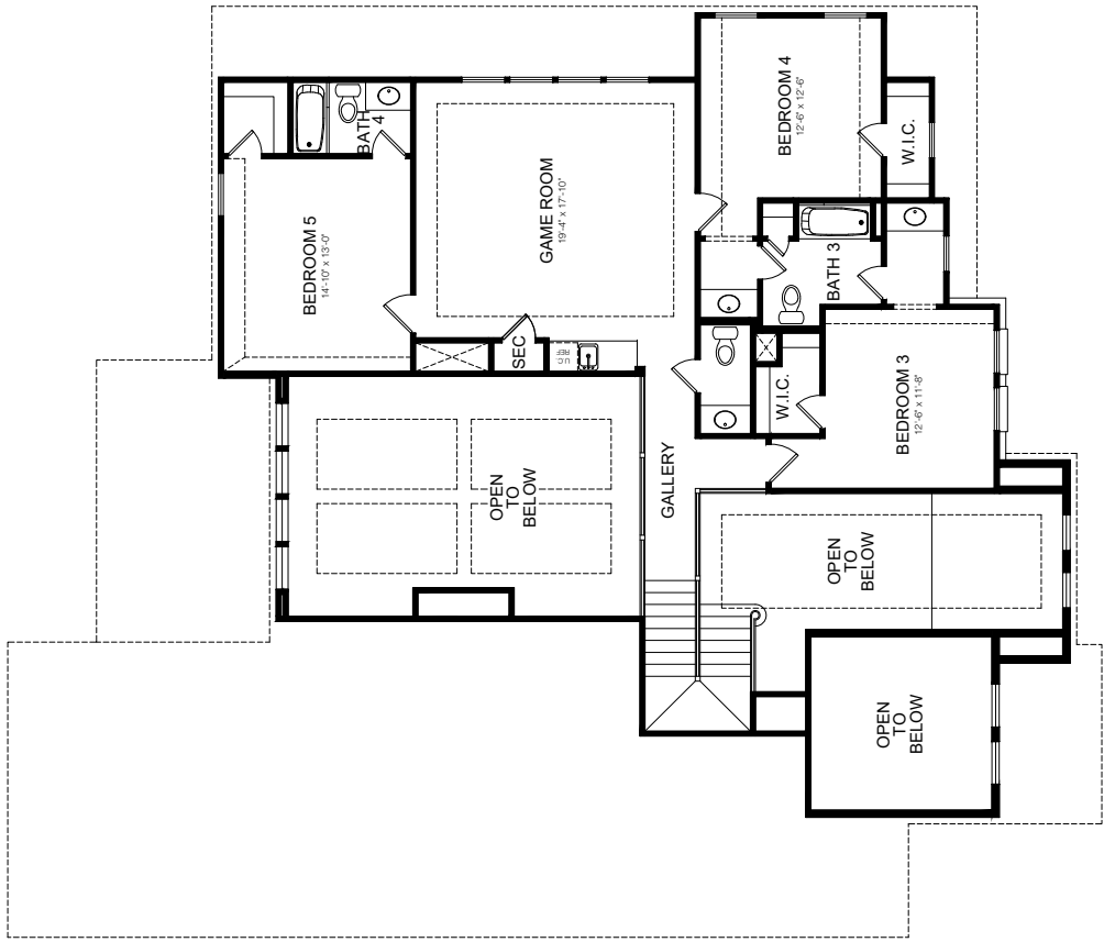
SECOND FLOOR PLAN ELEVATION A
