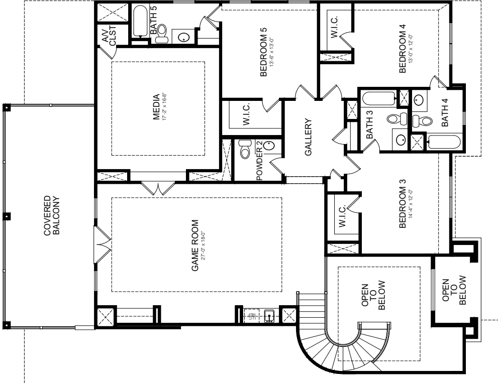
SECOND FLOOR PLAN ELEVATION A
