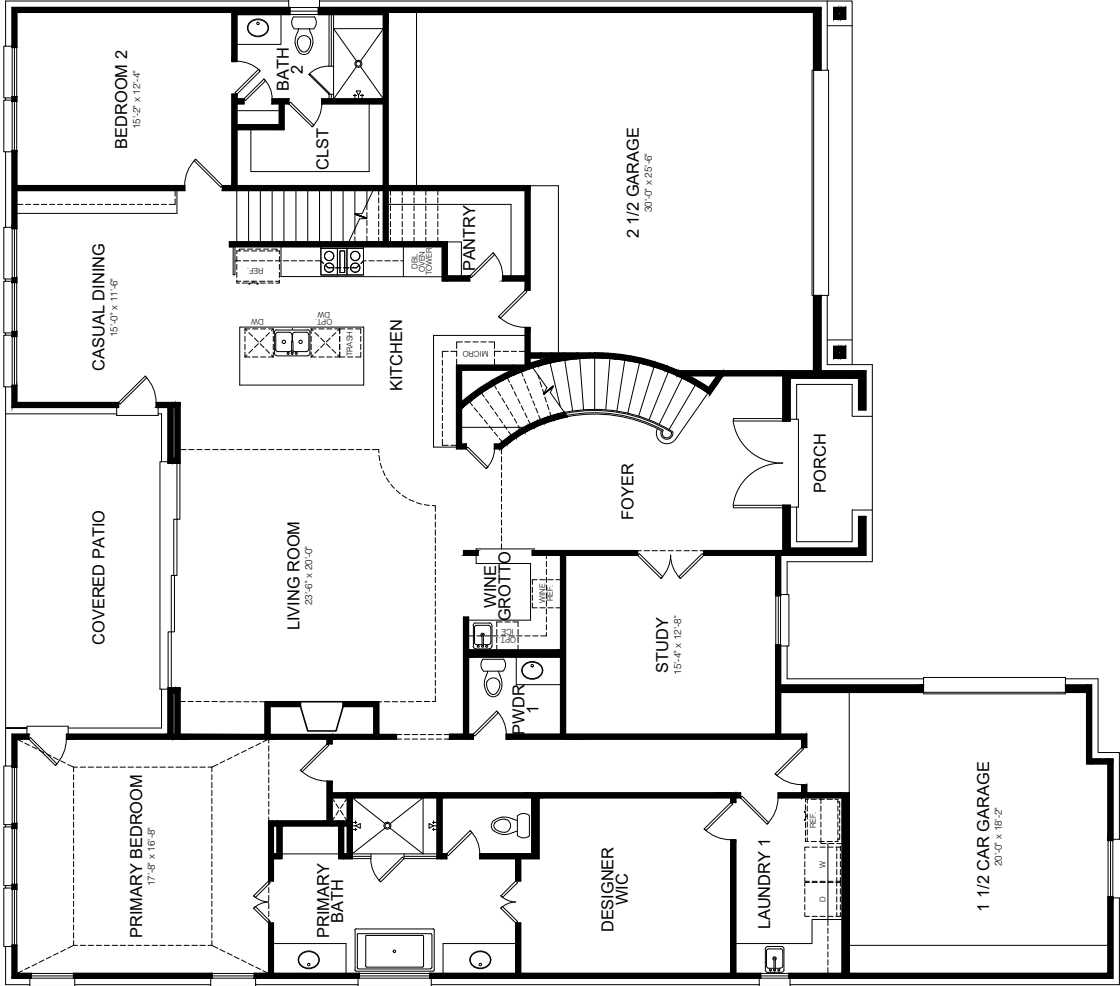
MAIN FLOOR PLAN ELEVATION A
