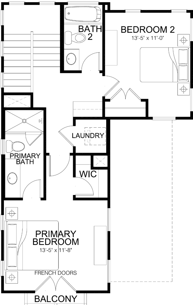
SECOND FLOOR PLAN ELEVATION A
