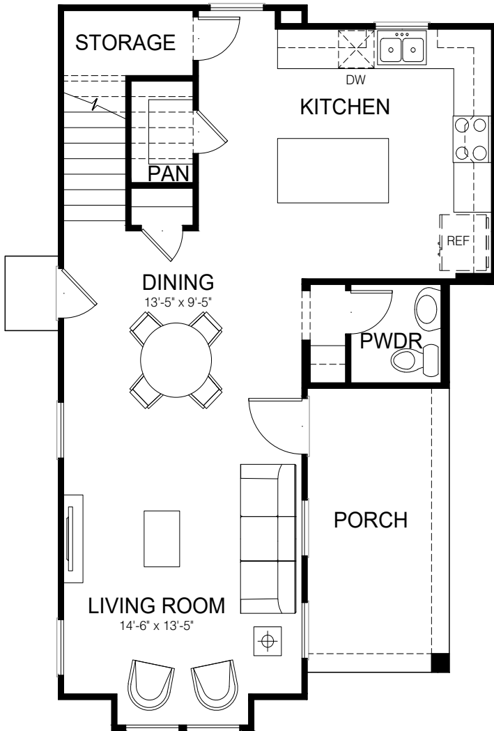
MAIN FLOOR PLAN ELEVATION A
