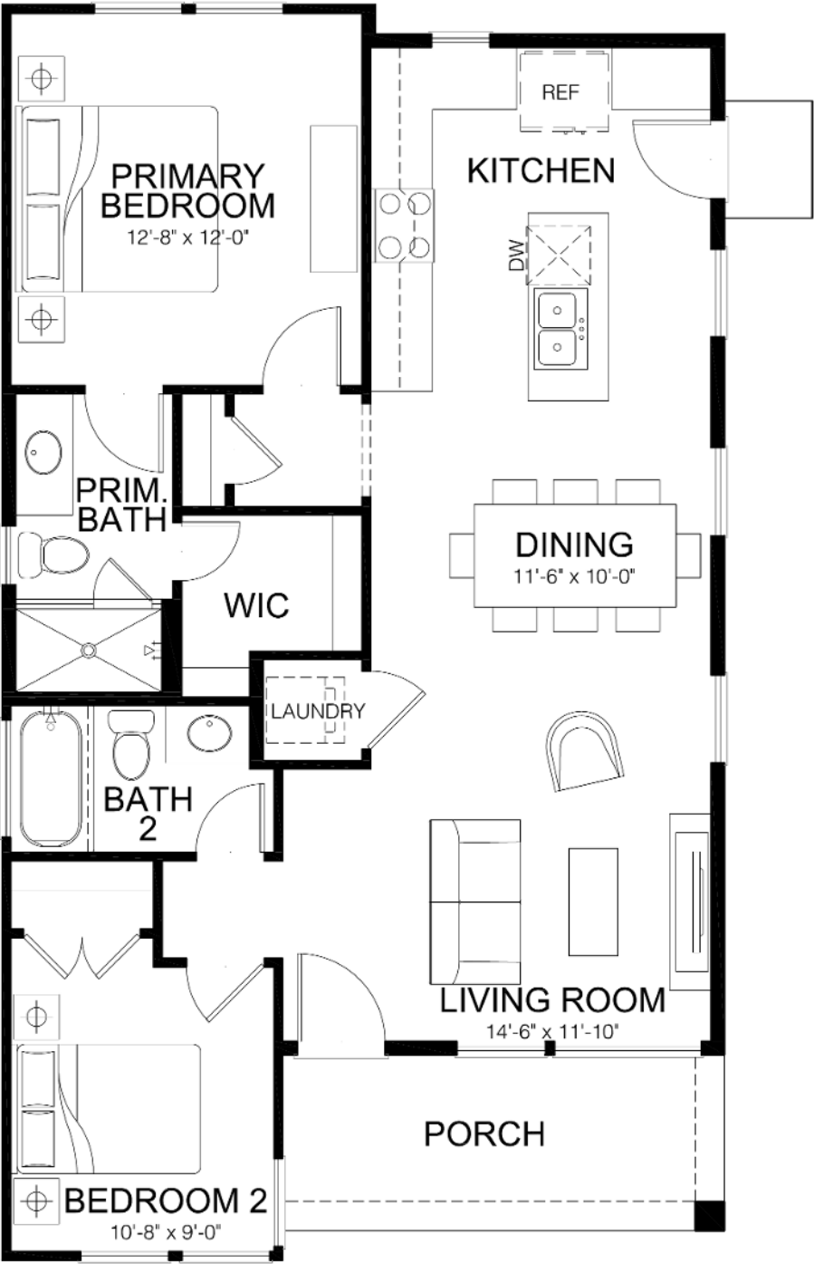
MAIN FLOOR PLAN ELEVATION A
