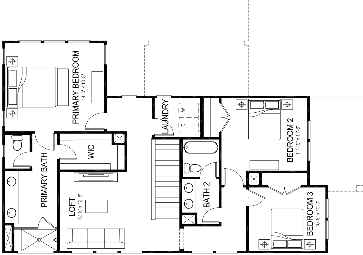
SECOND FLOOR PLAN ELEVATION A
