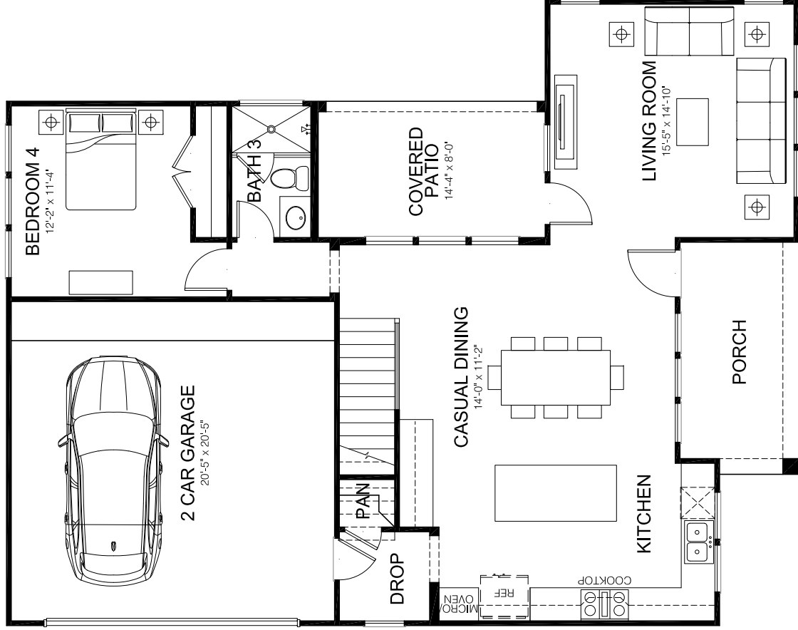
MAIN FLOOR PLAN ELEVATION A
