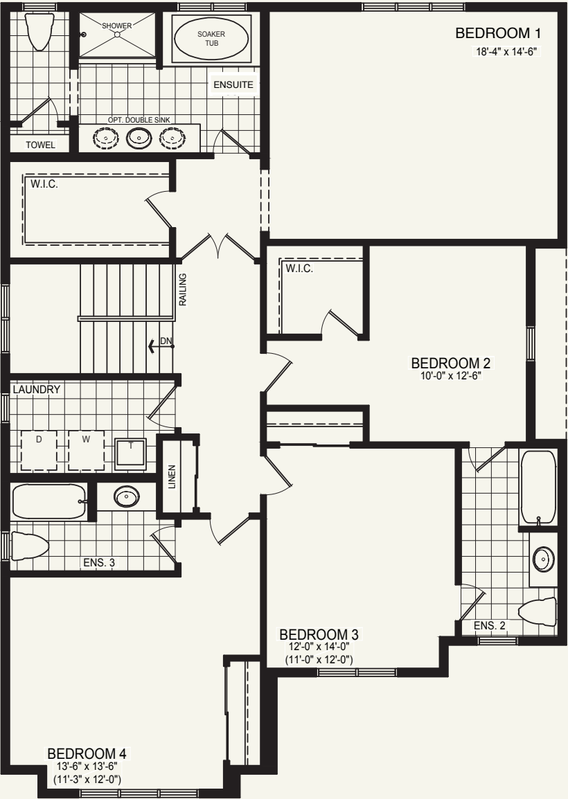
SECOND FLOOR PLAN STYLE A
