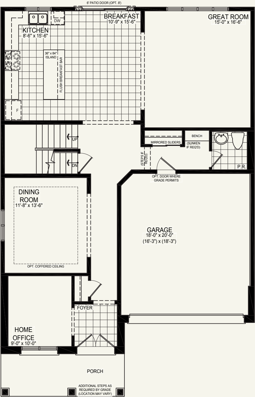
GROUND FLOOR PLAN STYLE A
