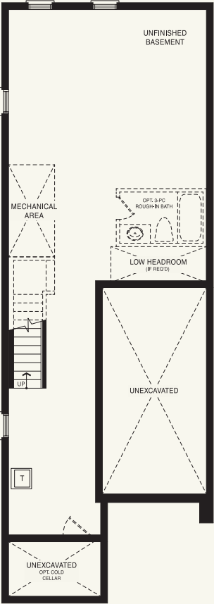
BASEMENT PLAN STYLE A
