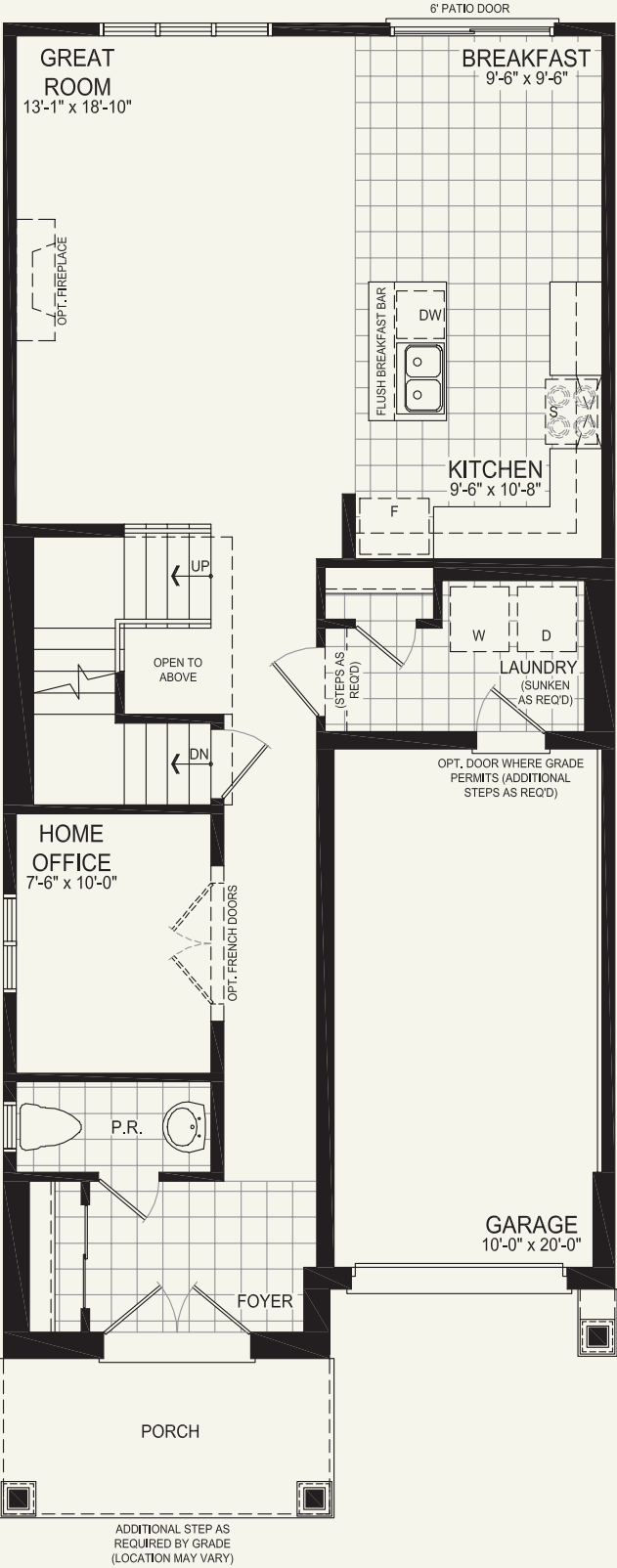
MAIN FLOOR PLAN STYLE A
