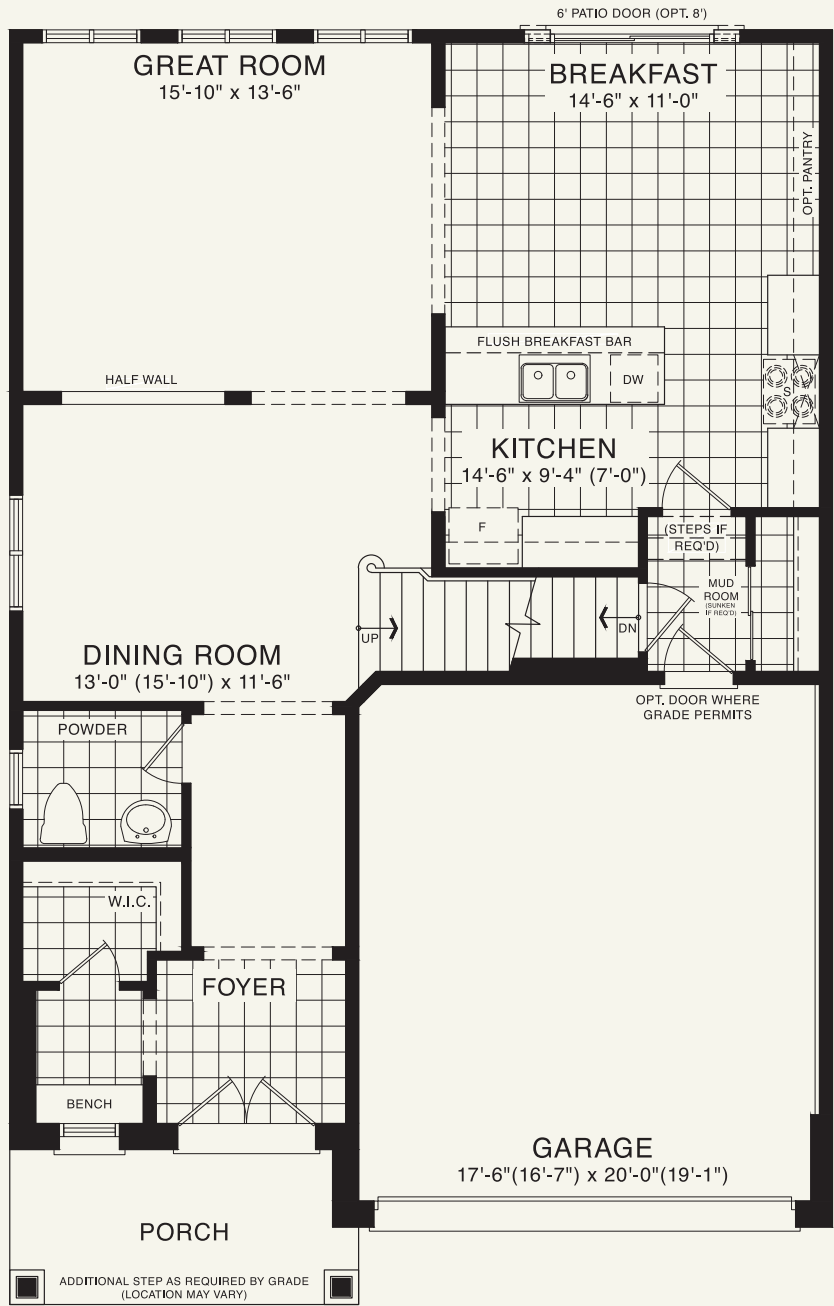
MAIN FLOOR PLAN STYLE A
