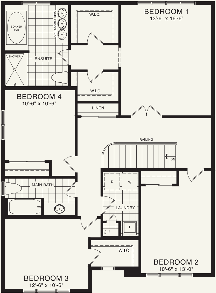
SECOND FLOOR PLAN STYLE A
