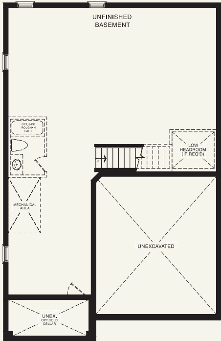
BASEMENT PLAN STYLE A
