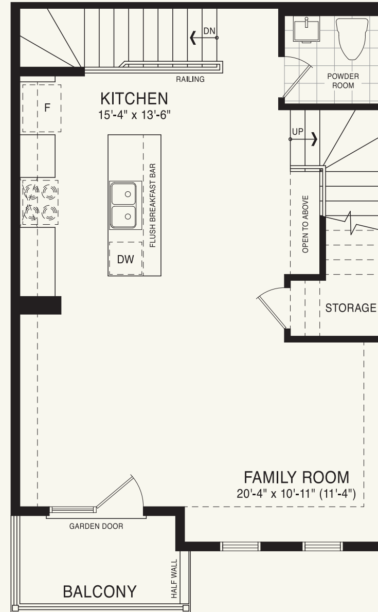
SECOND FLOOR PLAN STYLE A
