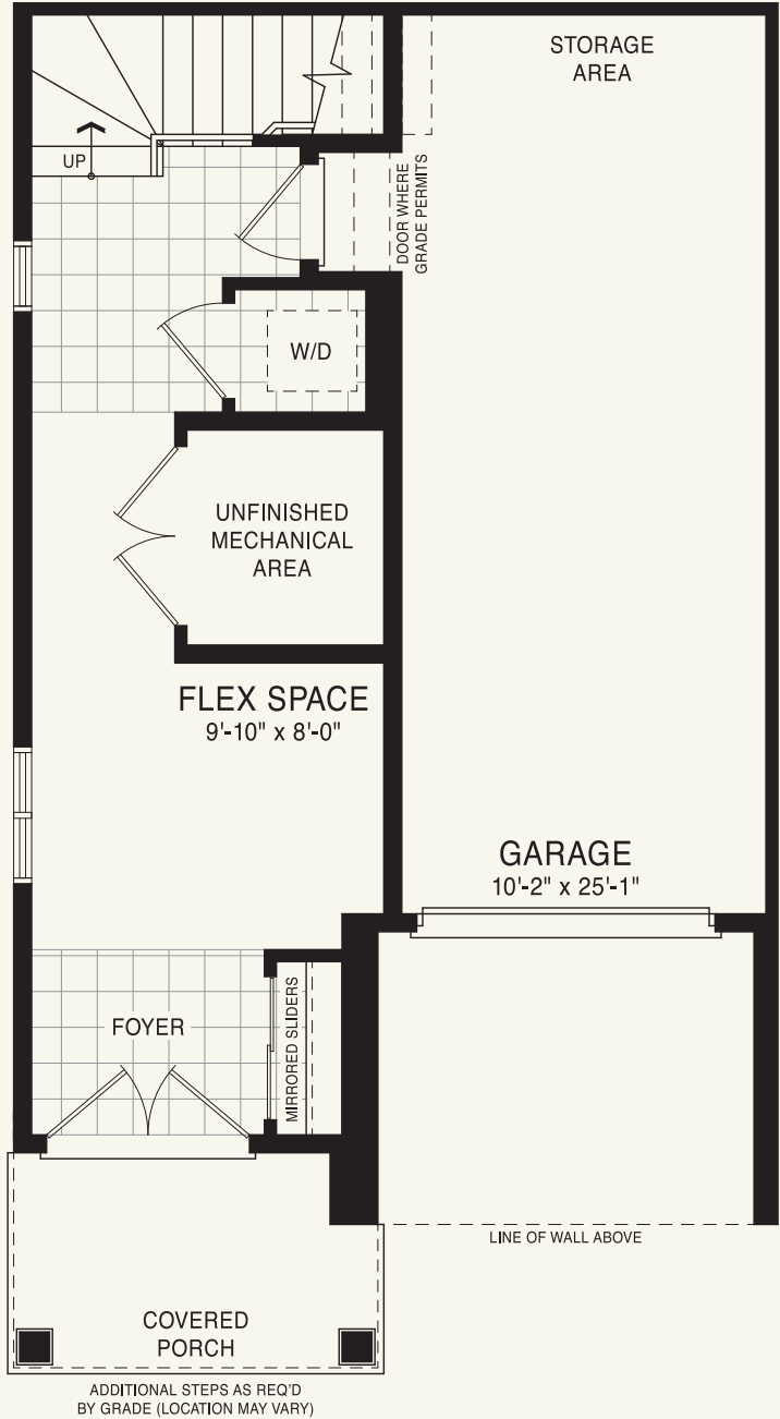
MAIN FLOOR PLAN STYLE A
