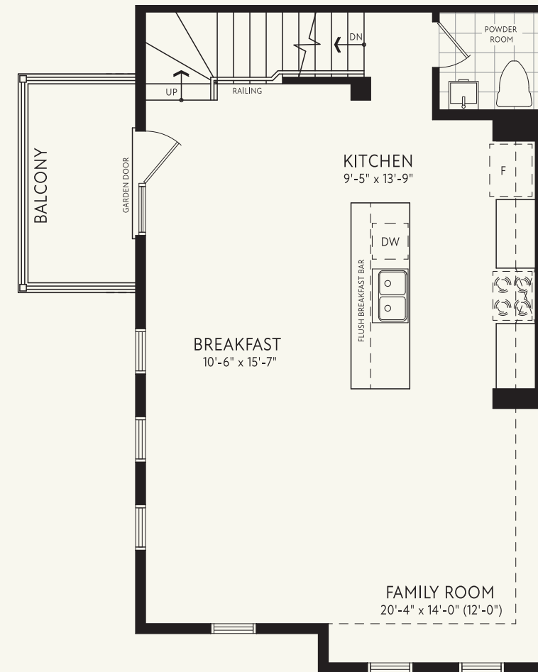
SECOND FLOOR PLAN STYLE A
