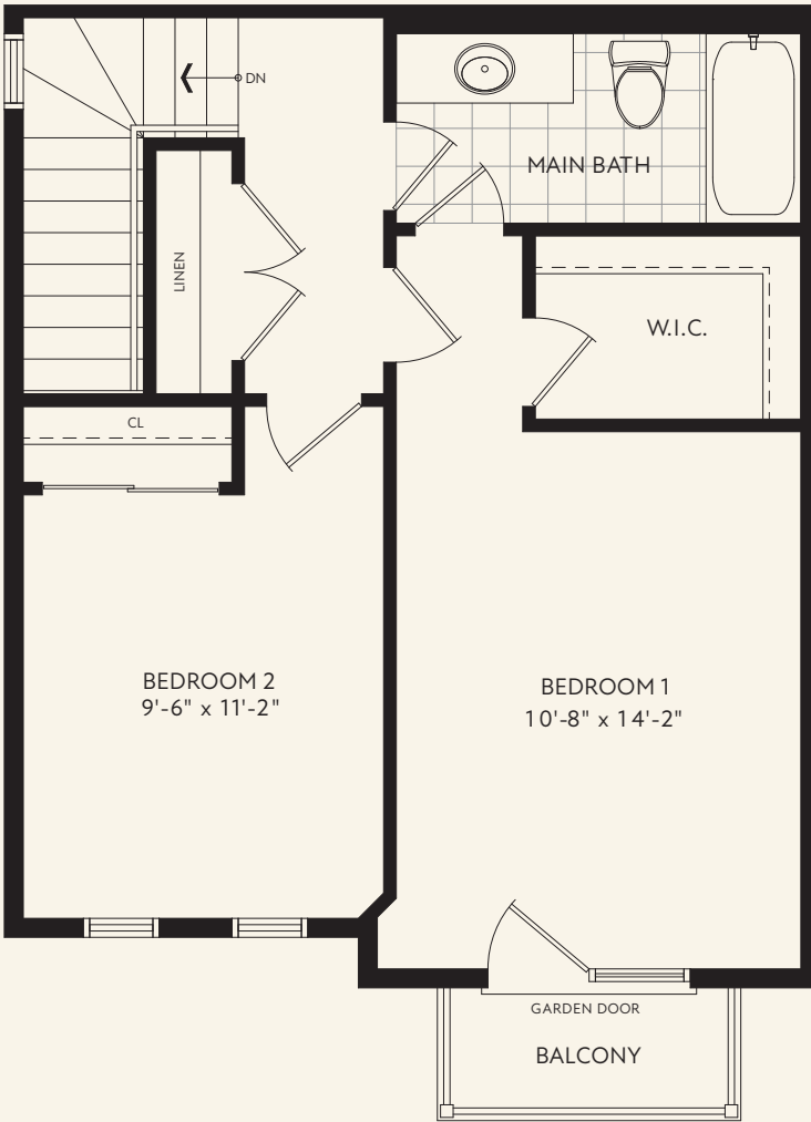
THIRD FLOOR PLAN CRAFTSMAN
