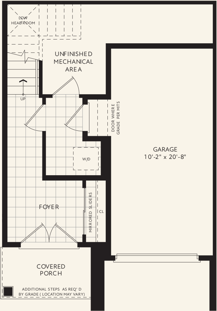
GROUND FLOOR PLAN CRAFTSMAN
