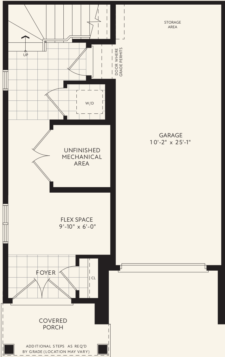
GROUND FLOOR PLAN CRAFTSMAN
