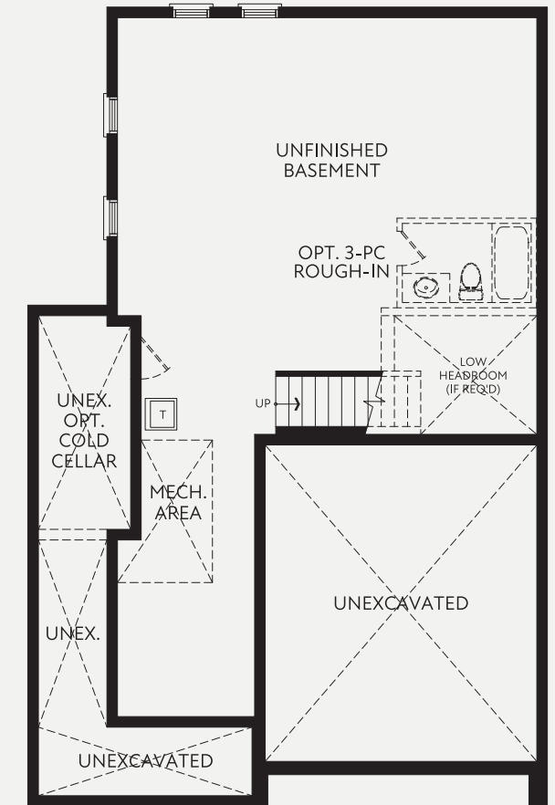
BASEMENT PLAN CRAFTSMAN
