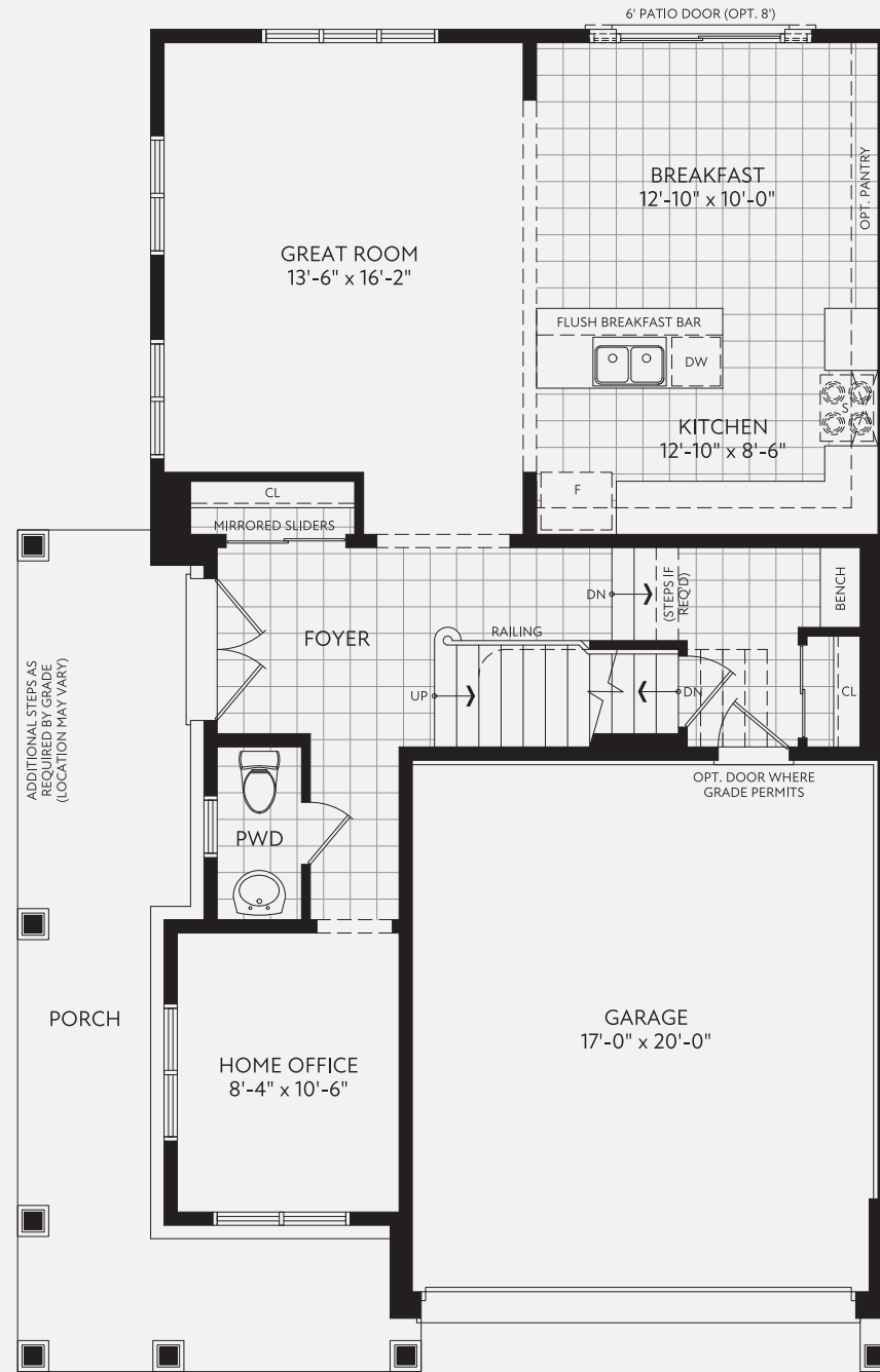
GROUND FLOOR PLAN CRAFTSMAN
