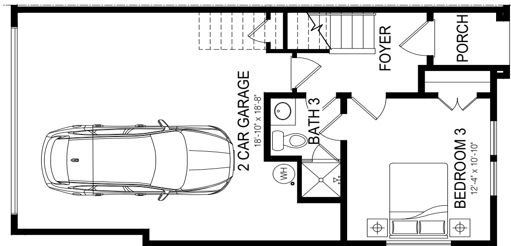
MAIN FLOOR PLAN ELEVATION A
