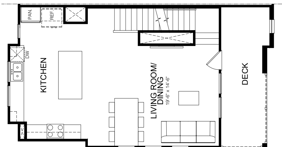
SECOND FLOOR PLAN ELEVATION A
