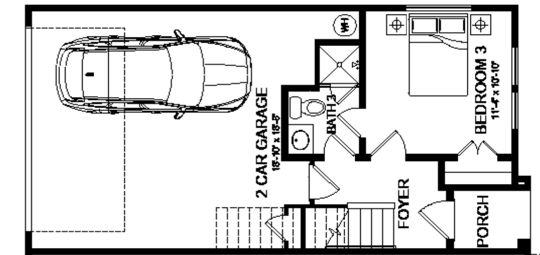
MAIN FLOOR PLAN ELEVATION A
