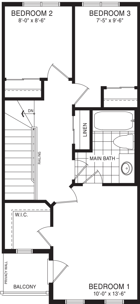
THIRD FLOOR PLAN ELEVATION A1
