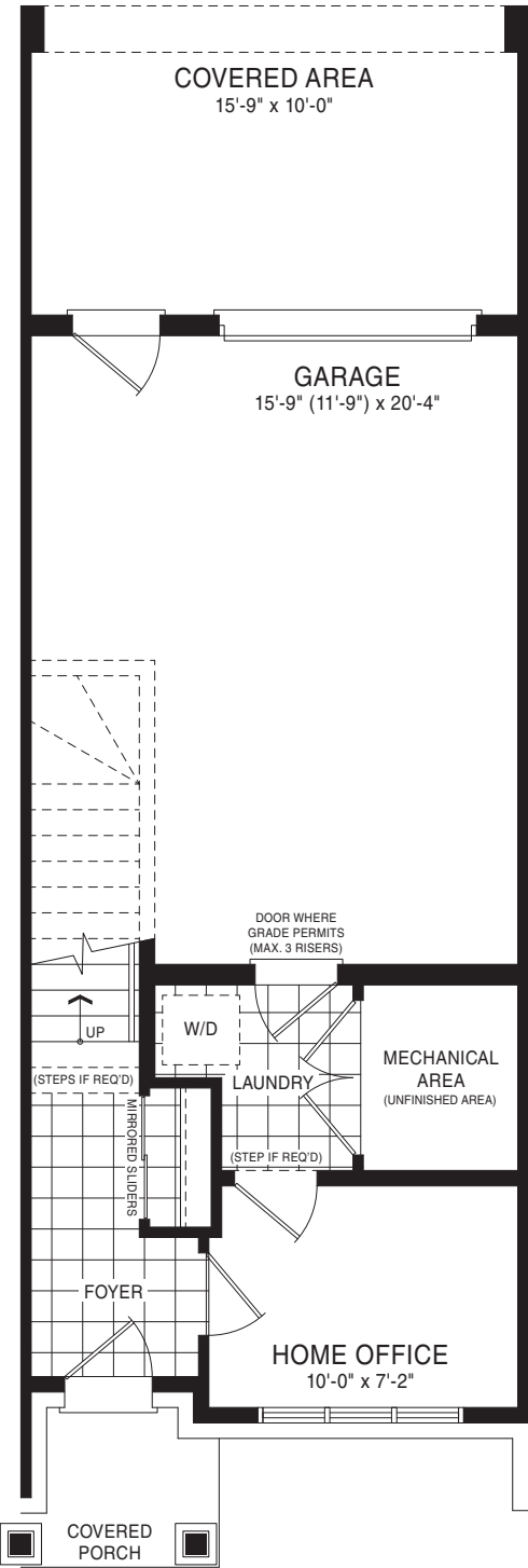
GROUND FLOOR PLAN ELEVATION A1
