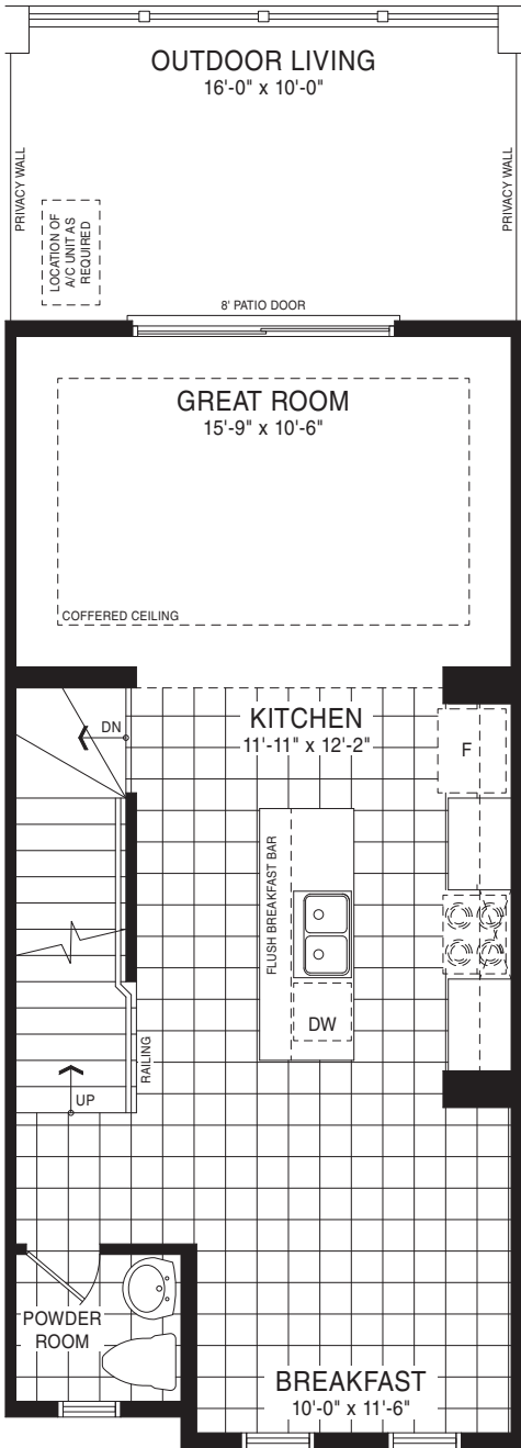
SECOND FLOOR PLAN ELEVATION A1
