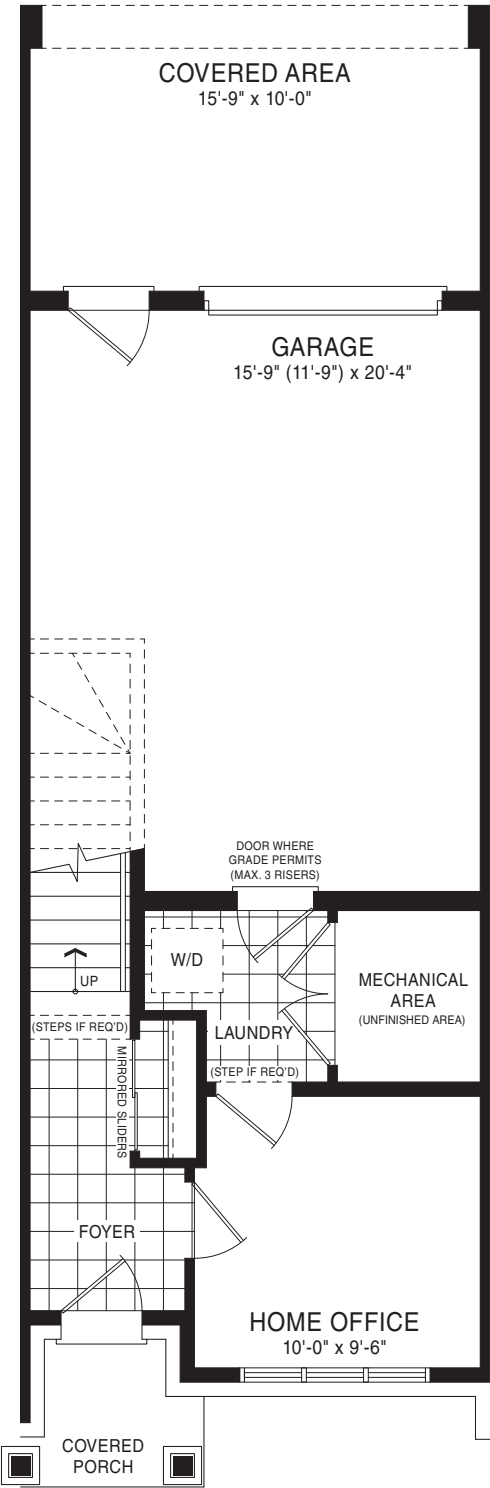
GROUND FLOOR PLAN ELEVATION A1
