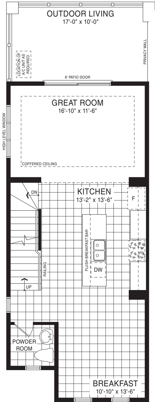
SECOND FLOOR PLAN ELEVATION A1
