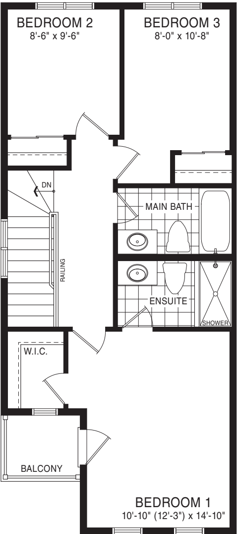
THIRD FLOOR PLAN ELEVATION A1
