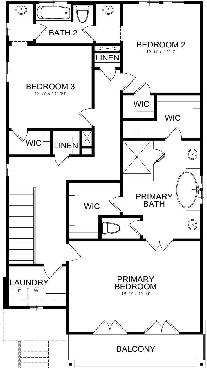
SECOND FLOOR PLAN ELEVATION A
