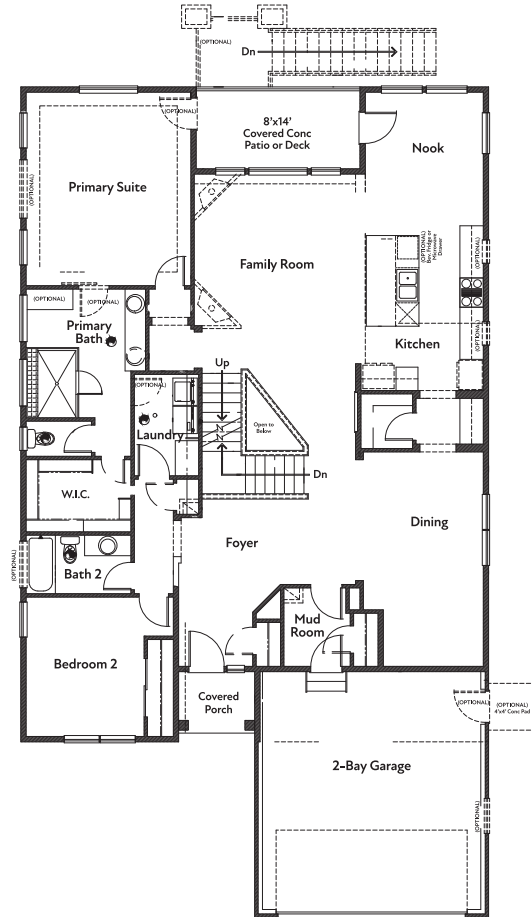
MAIN LEVEL FLOORPLAN
