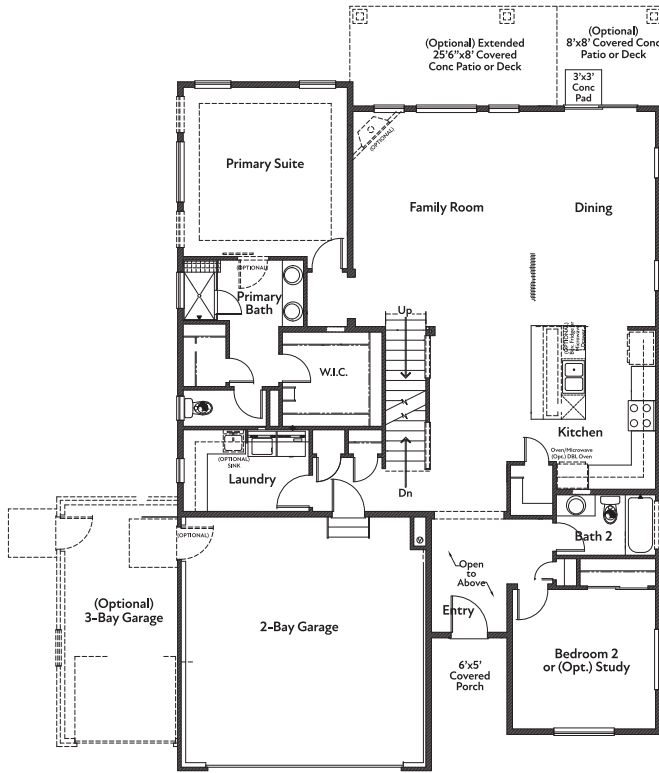
MAIN LEVEL FLOORPLAN
