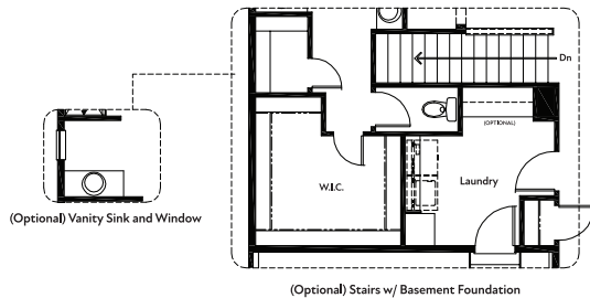
MAIN LEVEL FLOORPLAN
