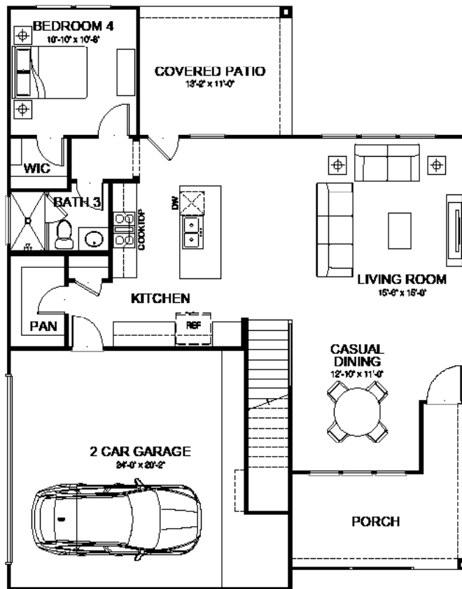
MAIN FLOOR PLAN ELEVATION A
