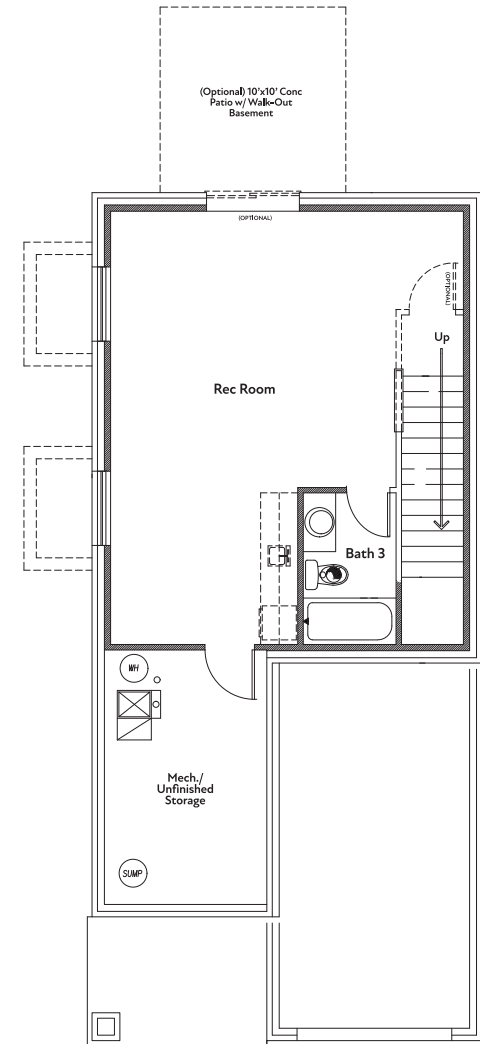
BASEMENT FLOORPLAN
