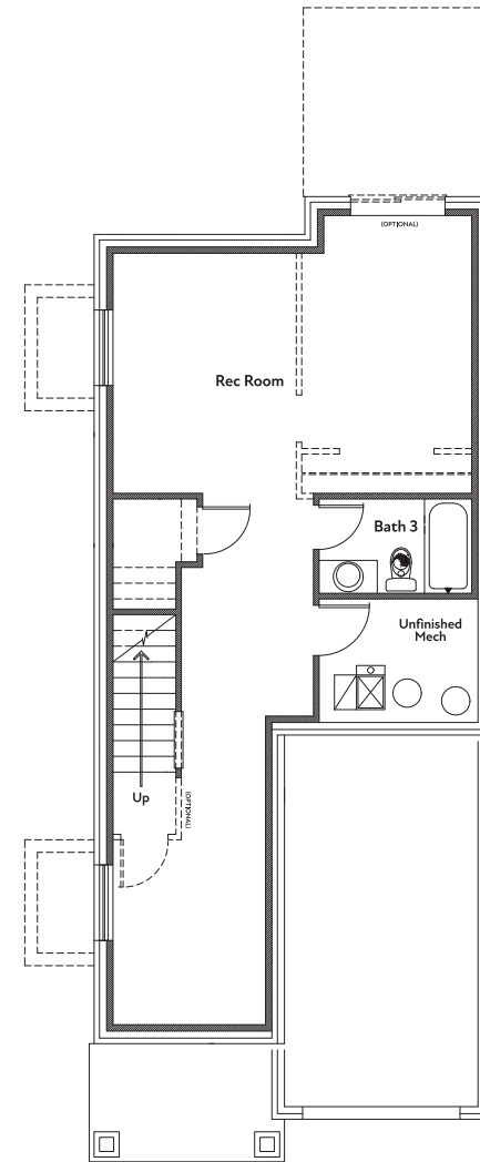
BASEMENT FLOORPLAN
