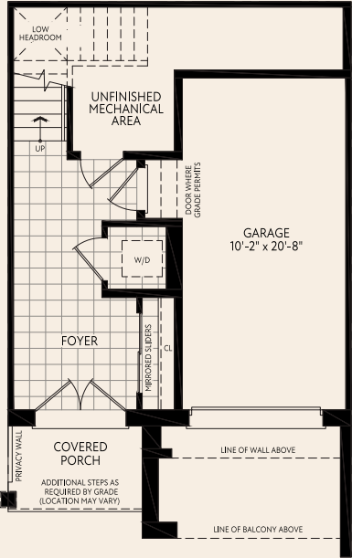
GROUND FLOOR PLAN MODERN 1
