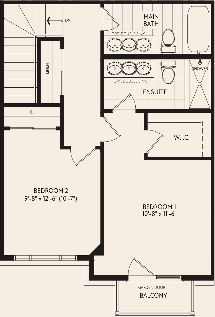
OPT. THIRD FLOOR PLAN MODERN 1
